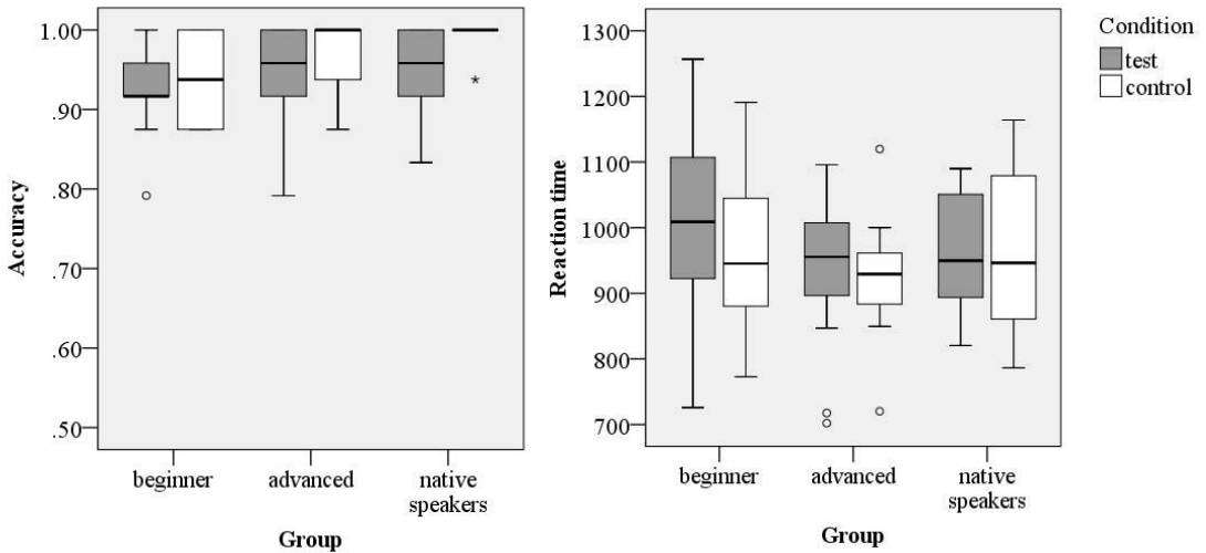
Figures 1 and 2: Mean accuracy (left) and reaction time (right) for the ABX-using length task on the test and control conditions in the three groups.
